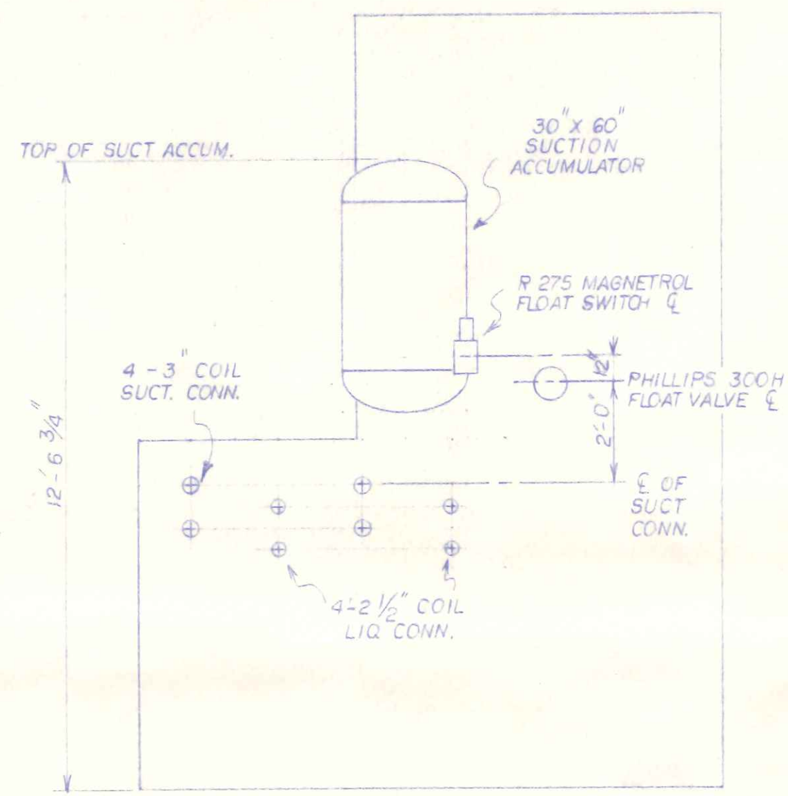
37013 NO-FROST SPRAY COOLER SIDE ELEVATION
